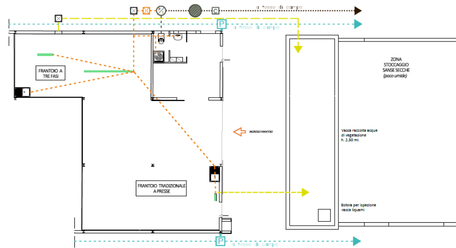
PIANO TERRA
